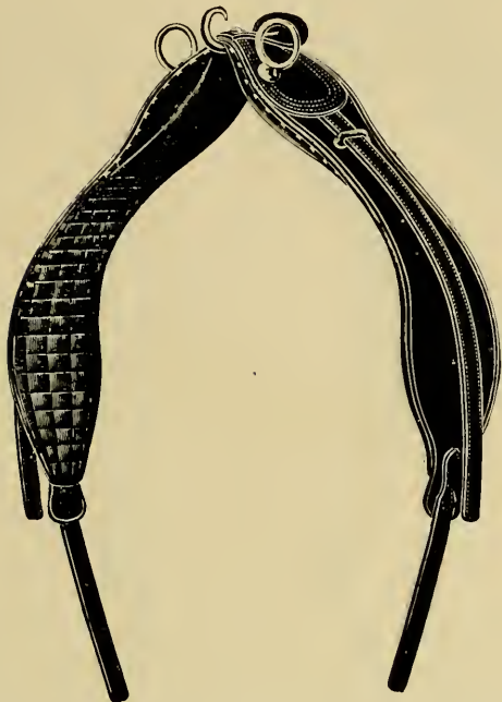
No. 375—Patent leather jockey; pannelled stitched, with terrets set ahead; double swell patent leather skirts, with coupe ends; four row stitched, running bearers, with metal or patent leather loops; enamel leather pad, finely quilted; covered seat; metal rim cantle. Untrimmed. Sizes 3\frac{1}{2} , 4, 4\frac{1}{2} and 5 inches.
